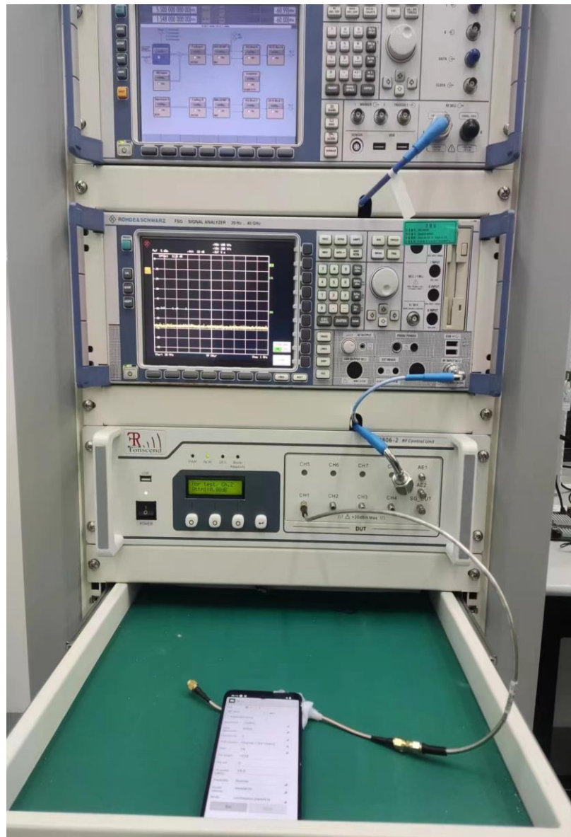
Figure: NII Test Set-up Photo
