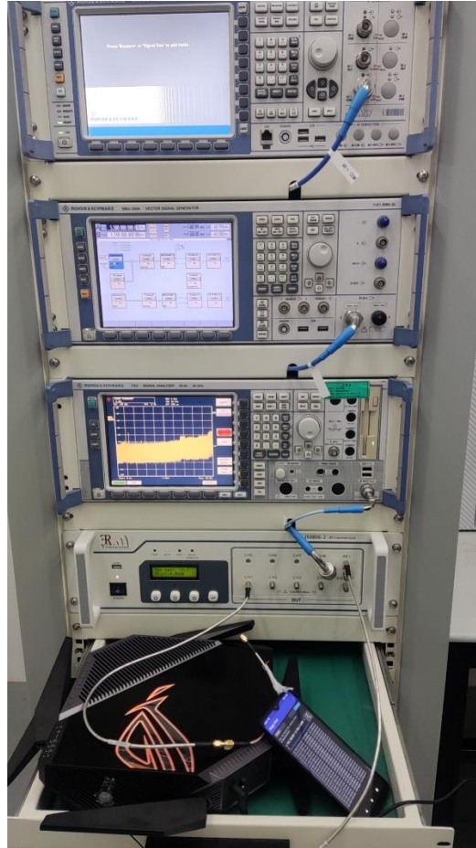
Figure: DFS Set-up Photo
