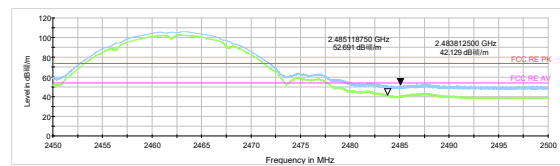
802.11b-Channel 11 Peak+ Average
