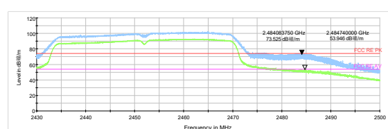
802.11n HT40 -Channel 9 Peak+ Average
