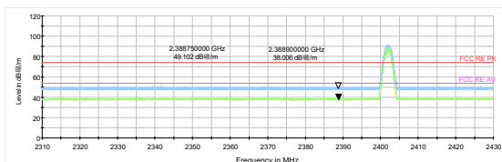
Bluetooth LE (1M) Channel 0 Peak+ Average
