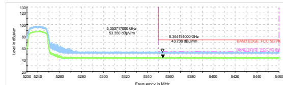
802.11a-Channel 48: Peak+Average
