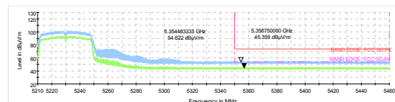
802.11n HT40-Channel 46: Peak+Average
