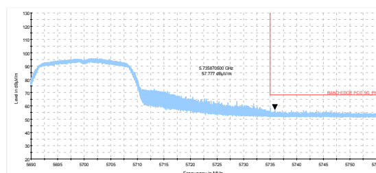
802.11n HT20-Channel 140: Peak
