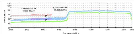
802.11ac VHT80-Channel 42: Peak+Average
