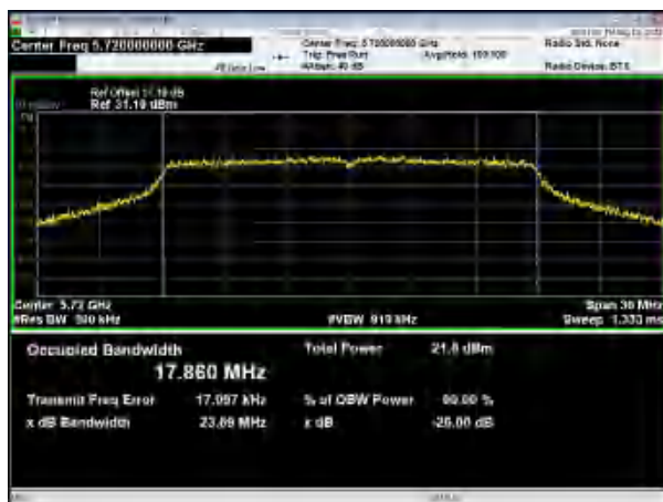
U-NII-3, 802.11n HT20, Channel No.: 144
