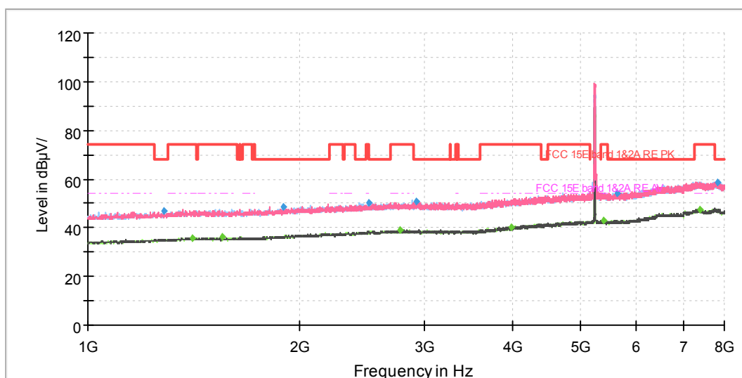
Radiates Emission from 1GHz to 8GHz
