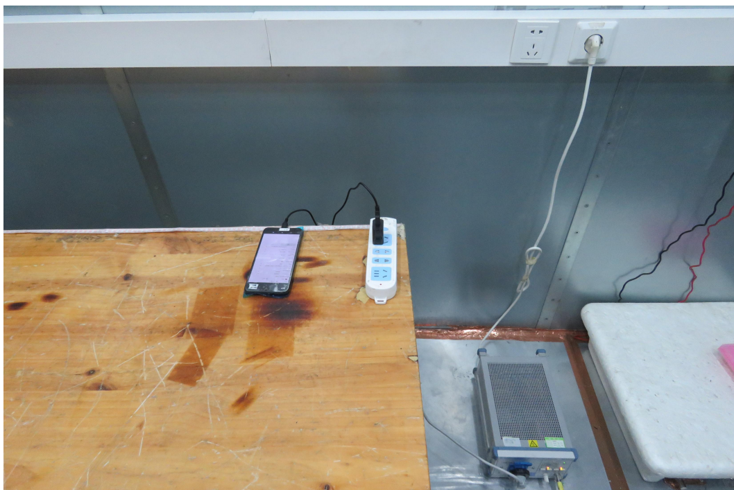
Picture 1 Conducted Emission Test Setup
