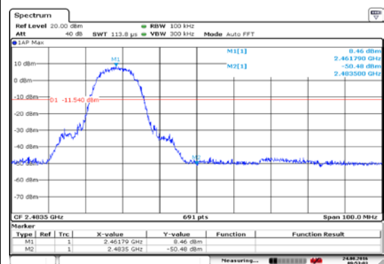
802.11b, Channel No.: 11
