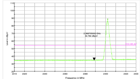
3DH5-Channel 0: Average
