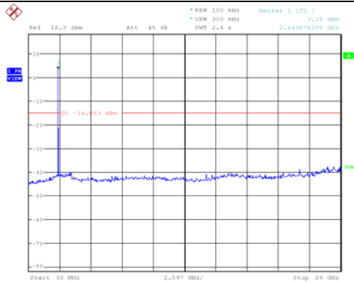
Conducted spurious emission: 8DPSK, Ch78, 30MHz~26GHz
