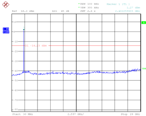
Conducted spurious emission: 8DPSK, Ch0, 30MHz~26GHz
