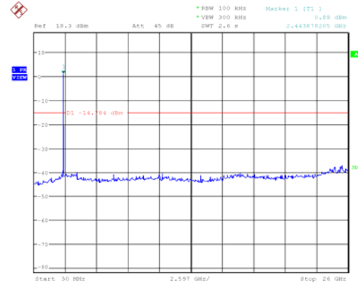
Conducted spurious emission: 8DPSK, Ch39, 30MHz~26GHz
