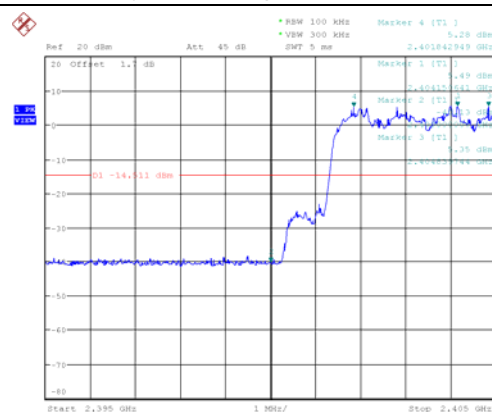
Frequency Band Edge: 8DPSK, Ch0, Hopping ON
