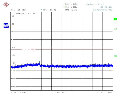
Channel 251: 1GHz~10GHz
