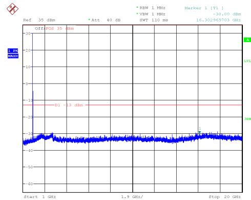
Channel 512: 1GHz~20GHz
