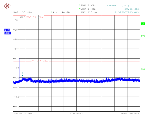
Channel 661: 1GHz~20GHz
