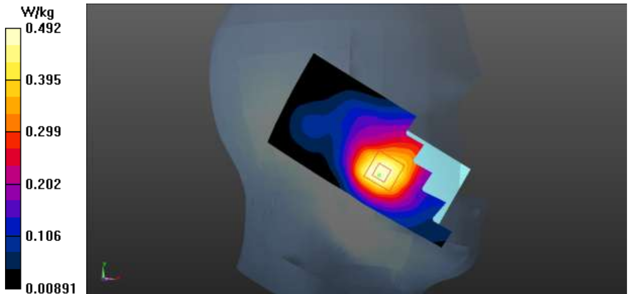
Fig.3 GSM 1900 Head
