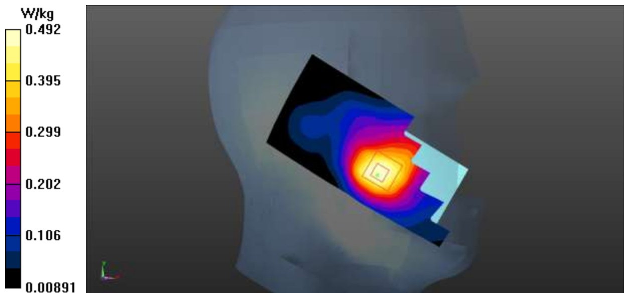
Fig.3 GSM 1900 Head
