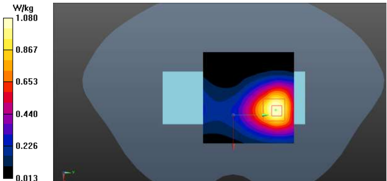
Fig.4 GSM 1900 Body
