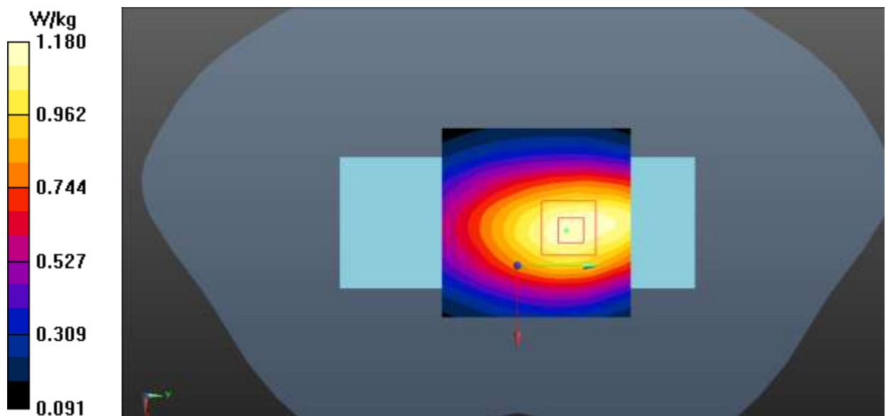
Fig.2 GSM 850 Body
