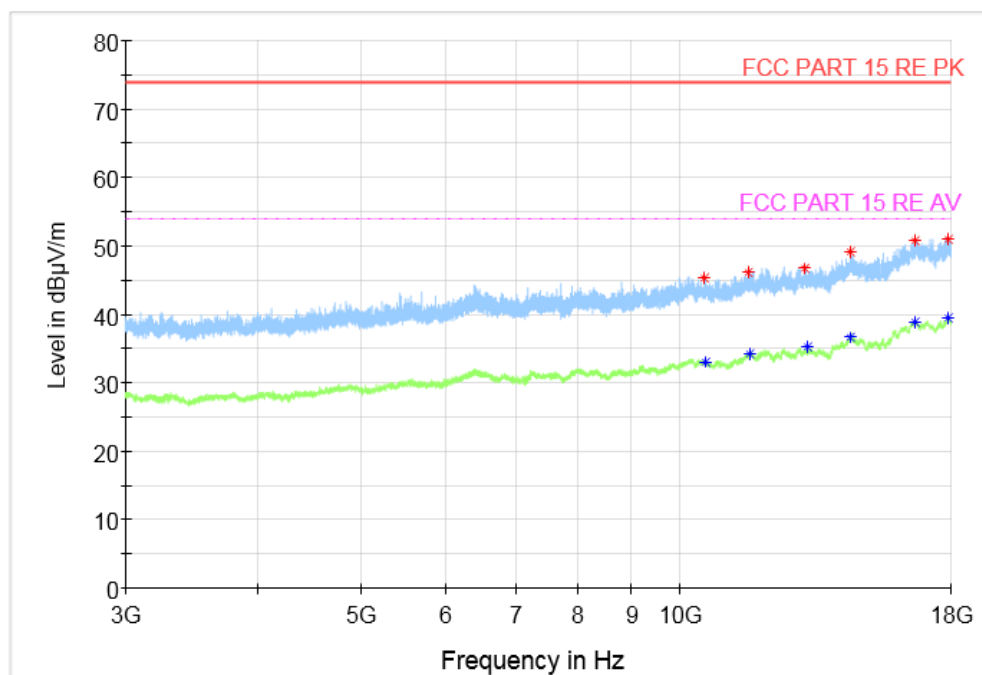
Fig.64 Radiated Spurious Emission (802.11n HT20, CH6, 3 GHz-18 GHz)
