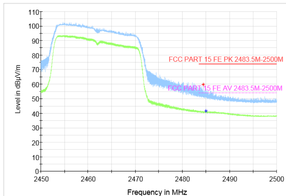
Fig.68 Radiated Restricted Band (802.11n HT20, CH11, 2.45GHz~2.5GHz)
