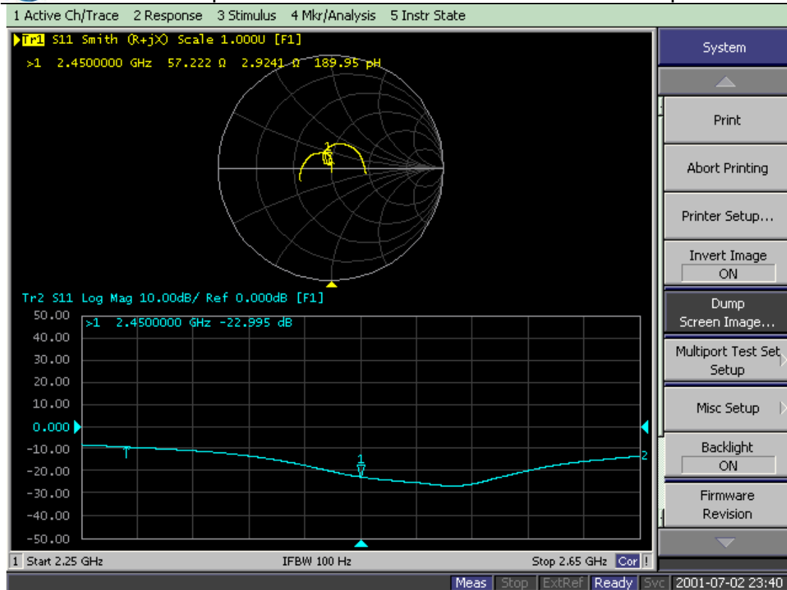
D2450V2-Head-8/28/2018
