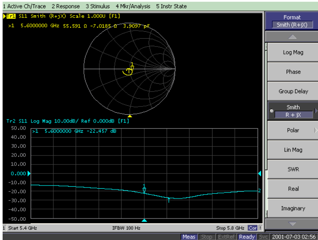
D5GHzV2-5600MHz -Body-1/4/2018
