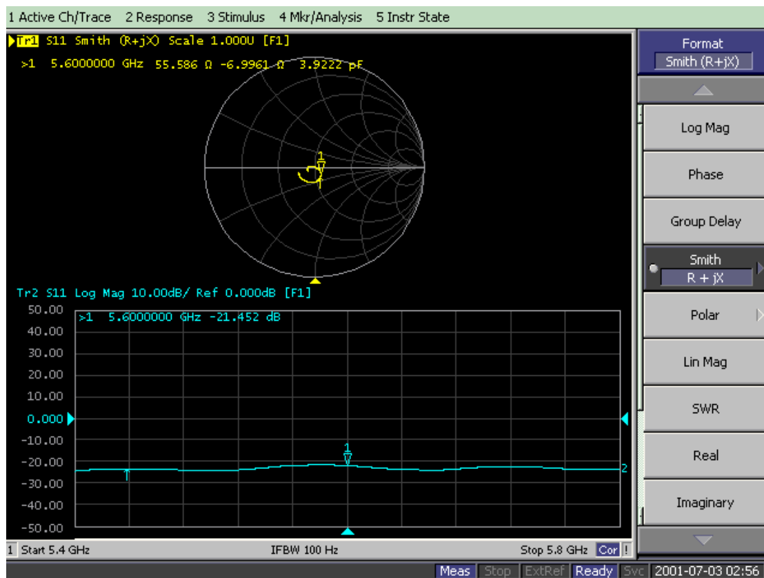
D5GHzV2-5600MHz-Head-1/4/2018
