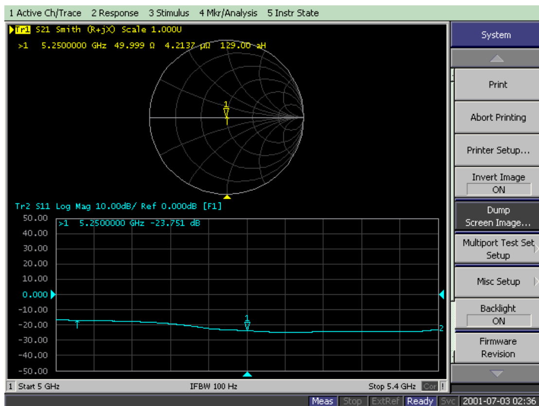
D5GHzV2-5250MHz -Body-1/4/2018
