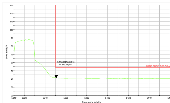
802.11a-Channel 64: Average
