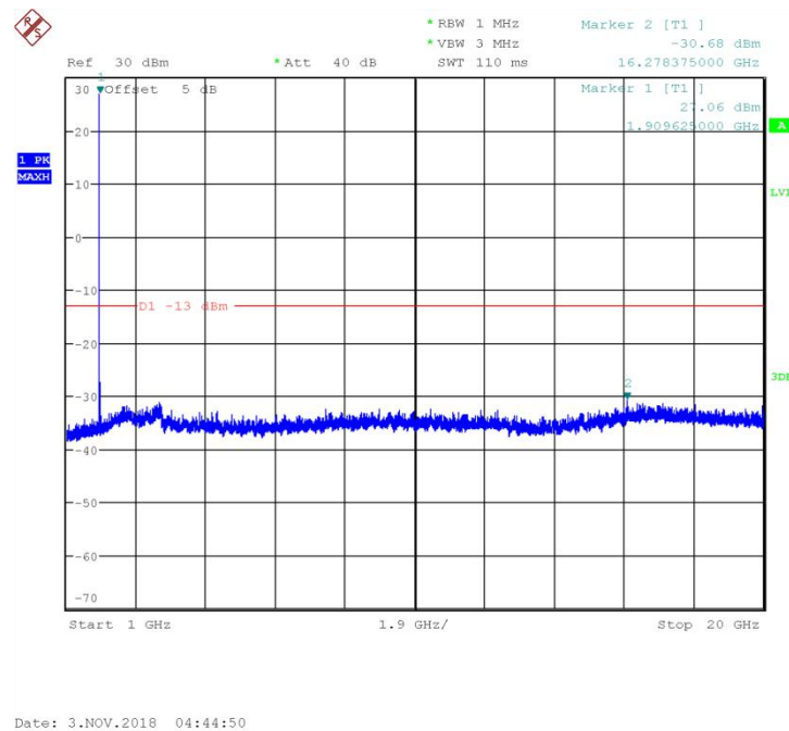
Fig.60 Channel 810: 1GHz~20GHz
