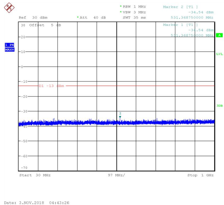
Fig.55 Channel 512: 30MHz~1GHz
