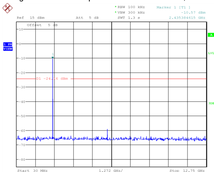
Fig.14 Conducted spurious emission: Ch19, 2440MHz
