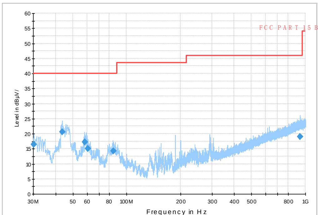
Fig.18 Radiated emission: Ch0, 30MHz~1GHz
