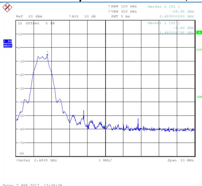
Fig.11 Frequency Band Edge: GFSK, Ch39, Hopping OFF
