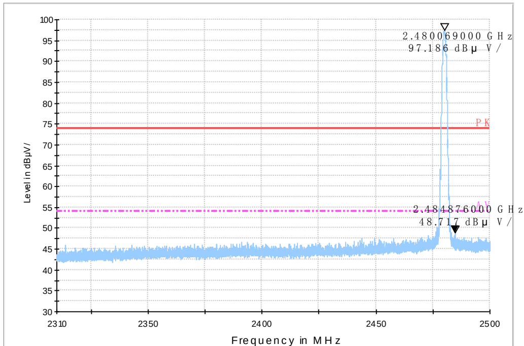
Fig.54 Radiated emission (Power): 8DPSK, high channel
