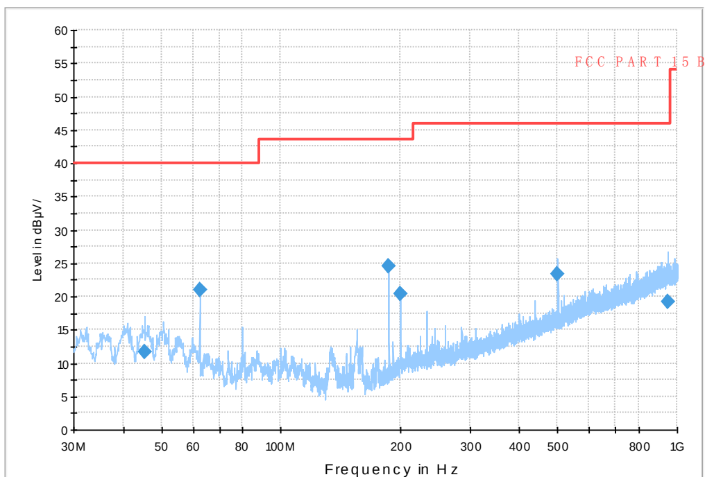
Fig.50 Radiated emission: 8DPSK, Ch0, 30MHz~1GHz
