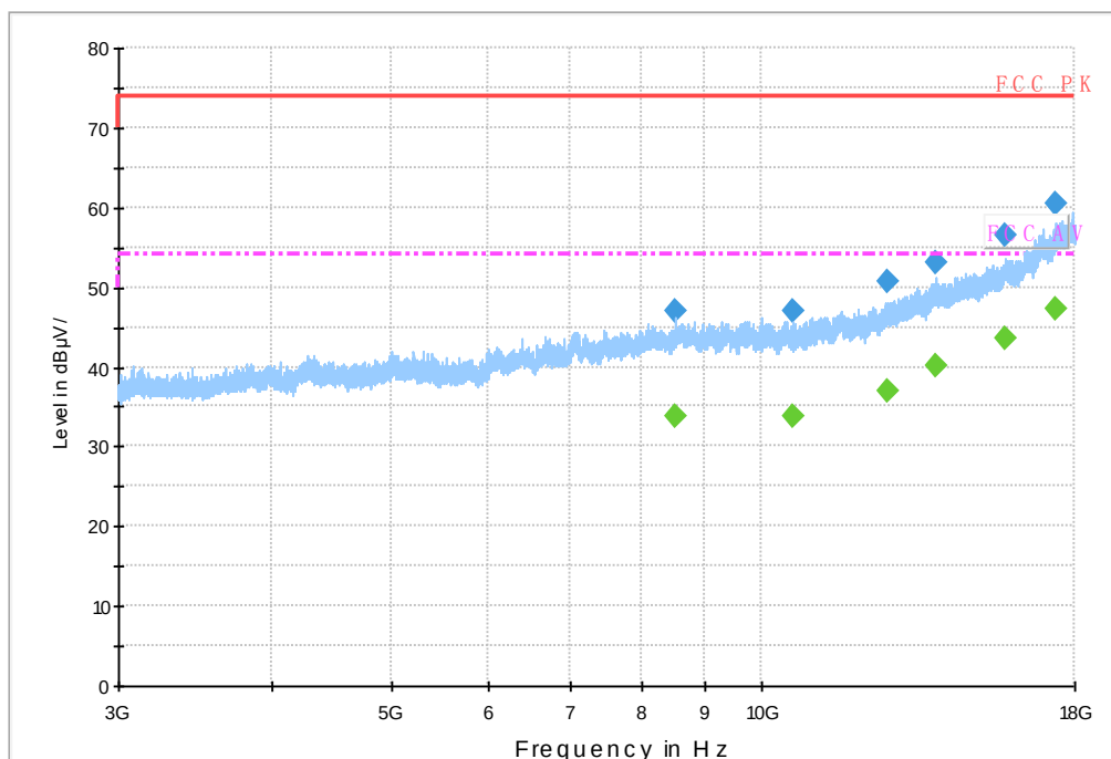
Fig.42 Radiated emission: GFSK, Ch0, 3GHz~18GHz
