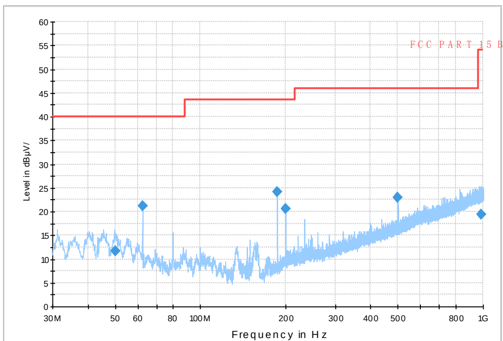
Fig.45 Radiated emission: \pi/4 DQPSK, Ch0, 30MHz~1GHz
