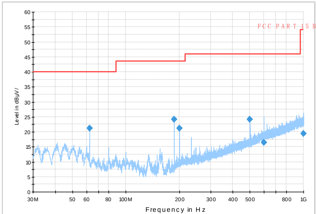
Fig.40 Radiated emission: GFSK, Ch0, 30MHz~1GHz
