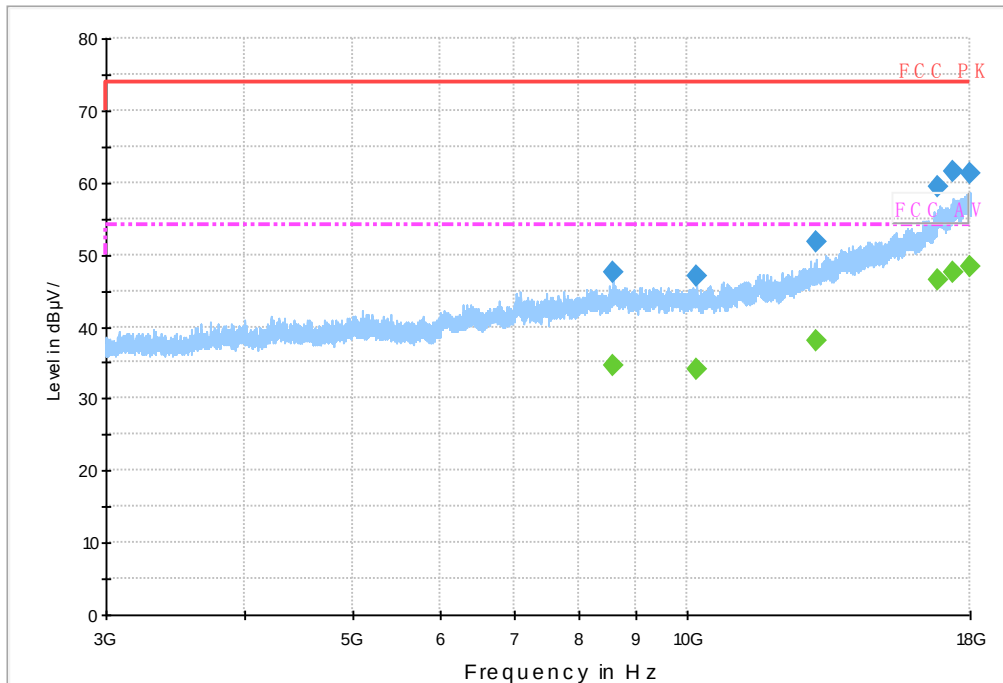
Fig.52 Radiated emission: 8DPSK, Ch0, 3GHz~18GHz
