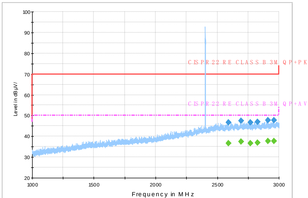
Fig.41 Radiated emission: GFSK, Ch0, 1GHz~3GHz
