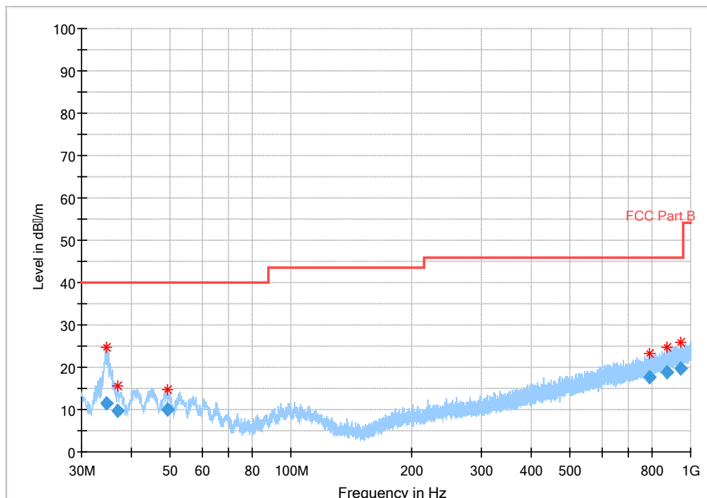
Fig.21 Radiated emission: Ch39, 30MHz~1GHz
