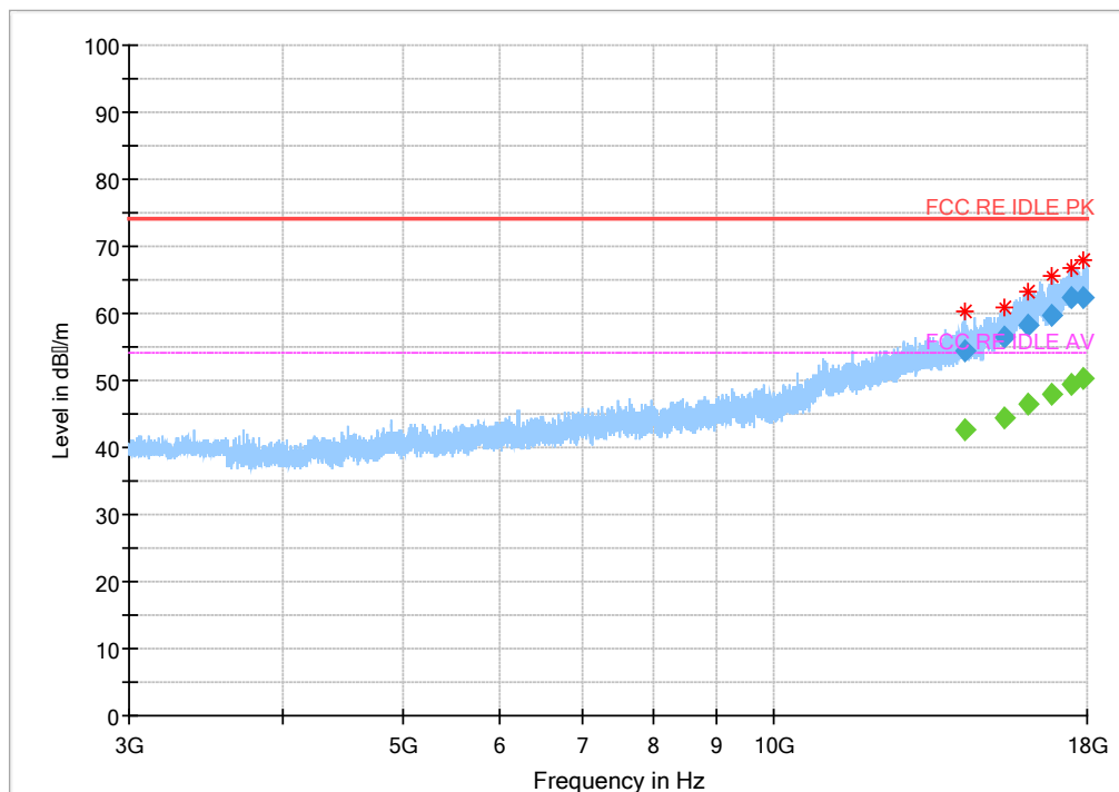
Fig.23 Radiated emission: Ch39, 3GHz~18GHz
