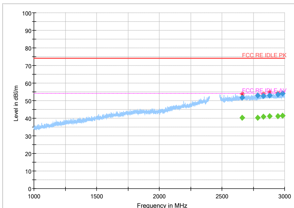
Fig.22 Radiated emission: Ch39, 1GHz~3GHz
