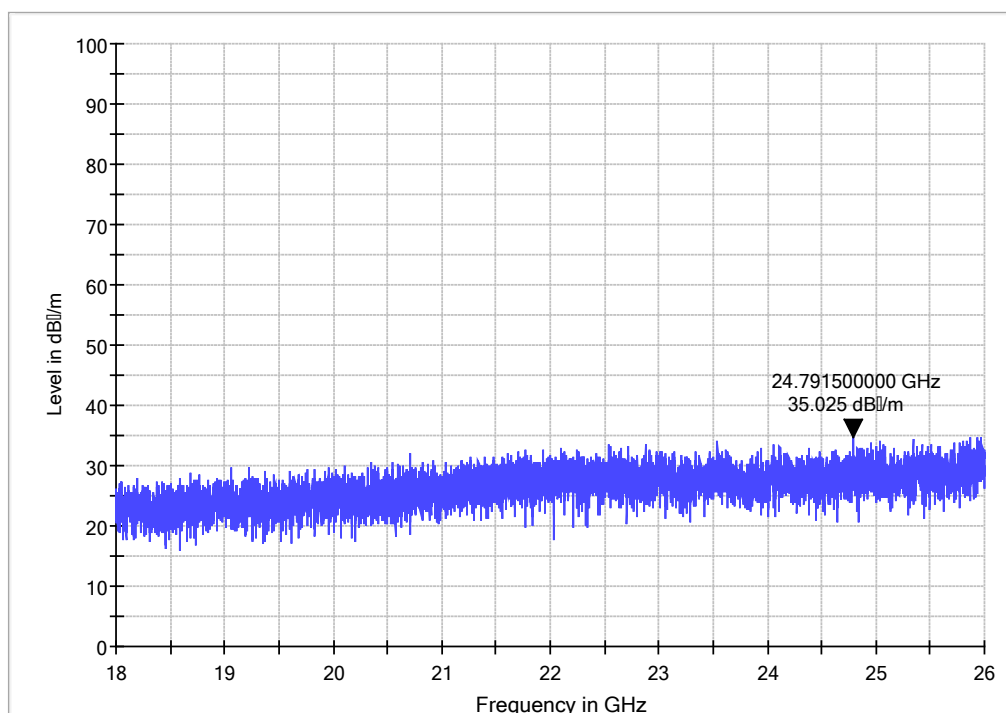
Fig.24 Radiated emission: Ch0, 18GHz~26GHz
