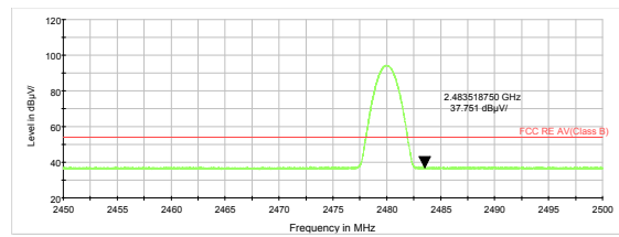
DH5-Channel 78: Average
