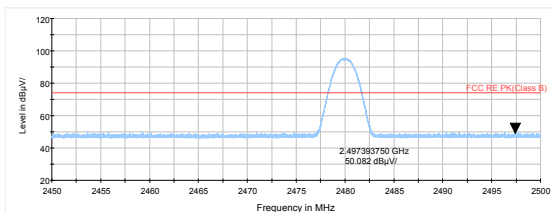
3DH5-Channel 78: Peak
