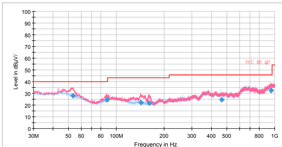
Radiates Emission from 30MHz to 1GHz
