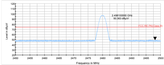
DH5-Channel 78: Peak
