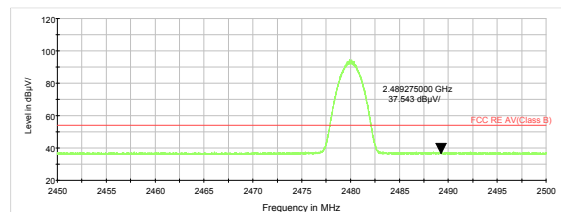
3DH5-Channel 78: Average
