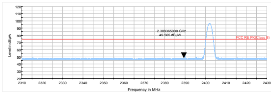
3DH5-Channel 0: Peak
