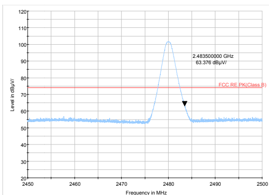
DH5-Channel 78: Peak
