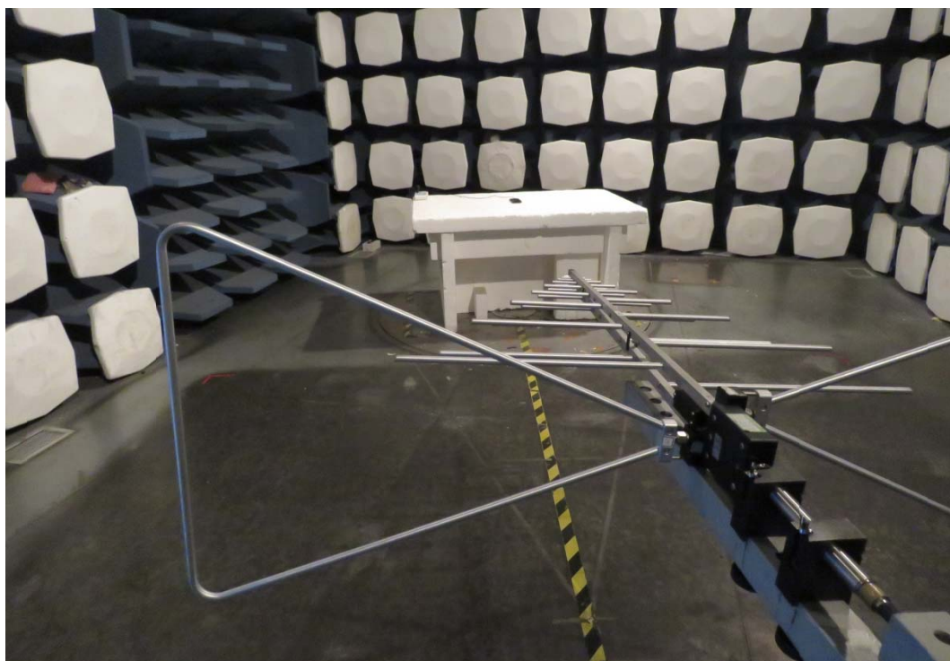
Below 1GHz
