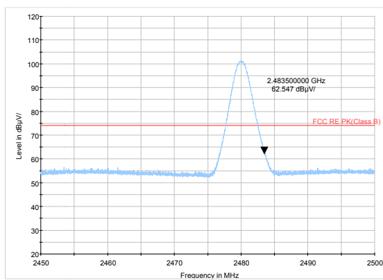
3DH5-Channel 78: Peak
