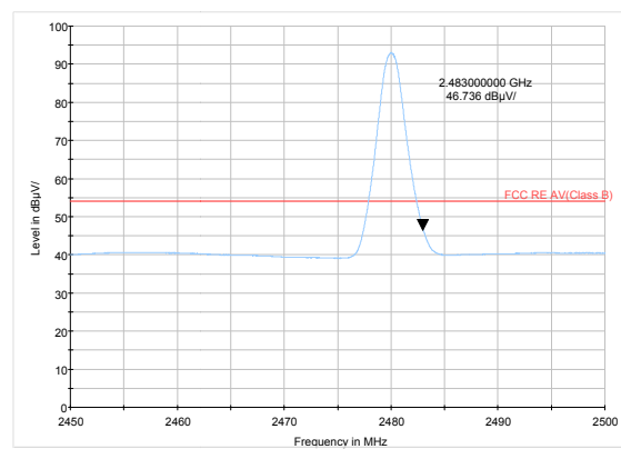
3DH5-Channel 78: Average
