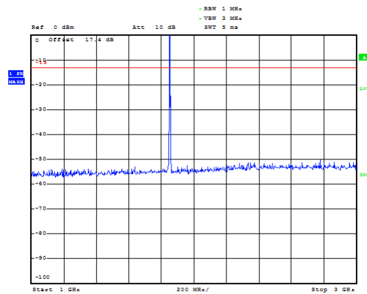
GPRS 1900 CH-Low 1GHz~3GHz
