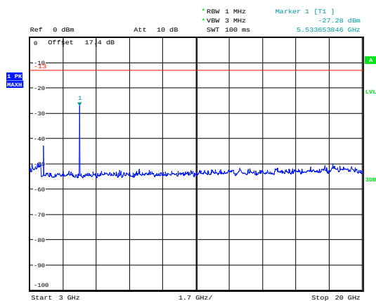
GPRS 1900 CH-Low 3GHz~20GHz
