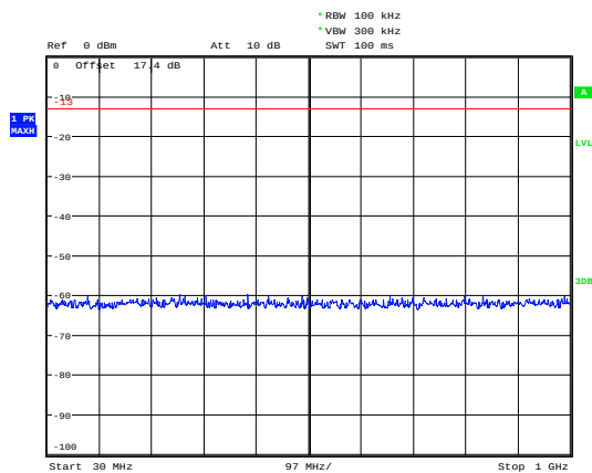
GPRS 1900 CH-Low 30MHz~1GHz
