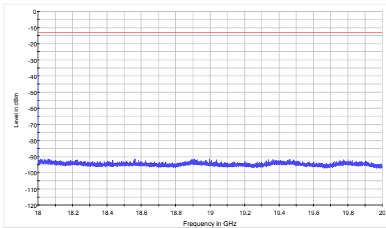
GSM 1900 CH-High 18GHz~20GHz
