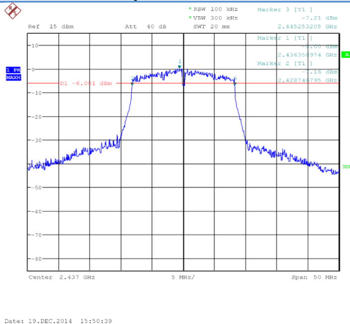
Fig.17 Occupied 6dB Bandwidth (802.11n-20MHz, Ch6)
