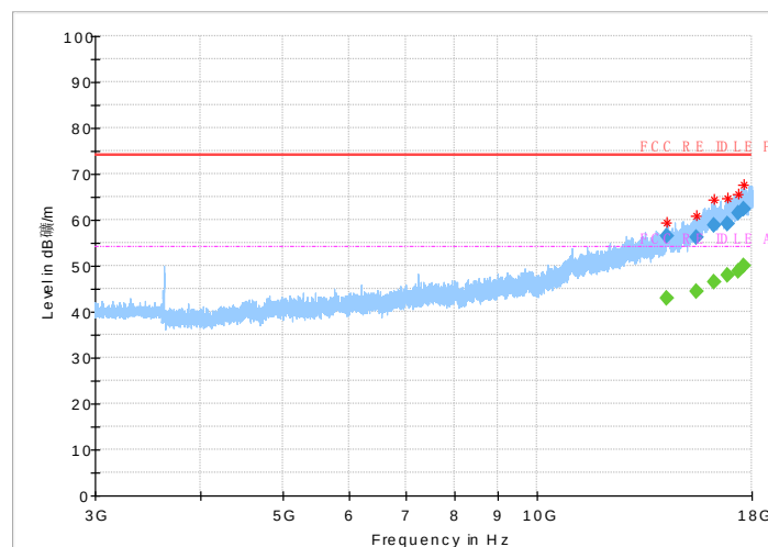
Fig.48 Radiated Spurious Emission (802.11b, Ch1, 3GHz~18GHz)
