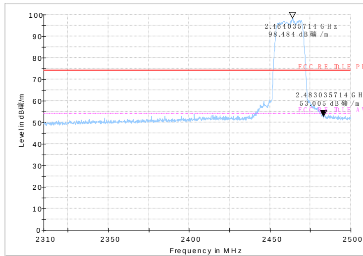
Fig.55 Radiated emission (Power): 802.11n, high channel
