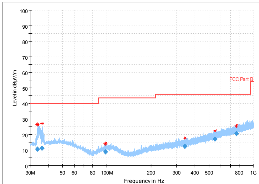
Fig.114 Radiated Spurious Emission (802.11 n-40MHz,Ch9,30MHz~1GHz)
