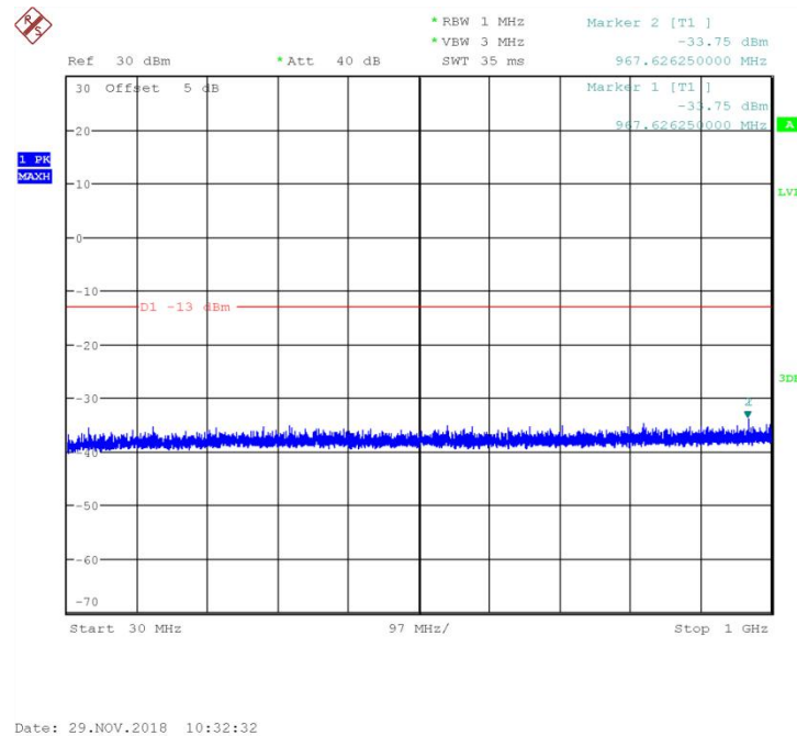
Fig.23 Channel 512: 30MHz~1GHz
