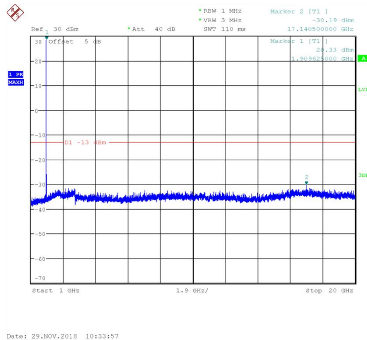
Fig.28 Channel 810: 1GHz~20GHz
