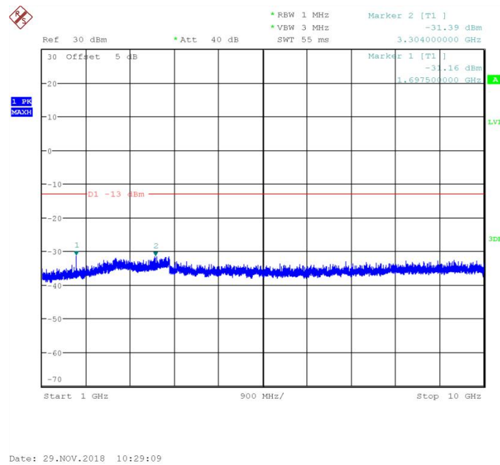
Fig.22 Channel 251: 1GHz~10GHz
