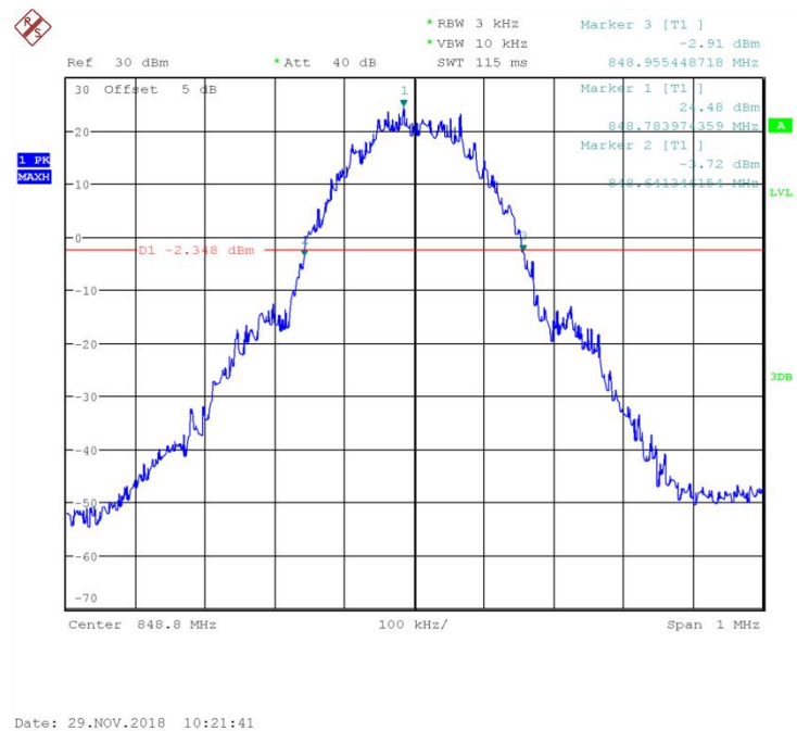
Fig.9 Channel 251- Emission Bandwidth (-26dBc BW)
