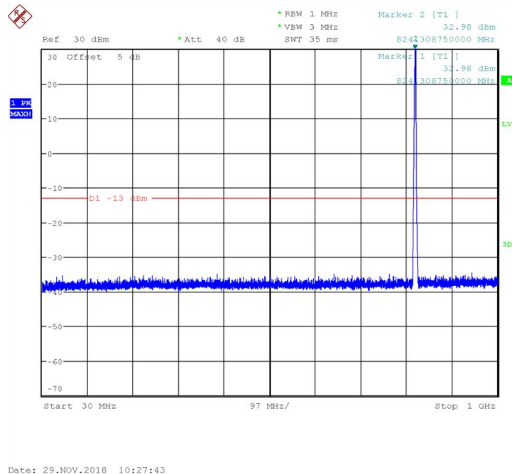
Fig.17 Channel 128: 30MHz~1GHz
