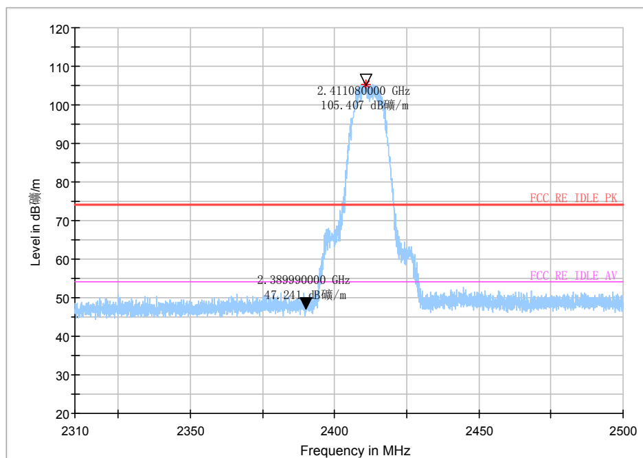
Peak detector
