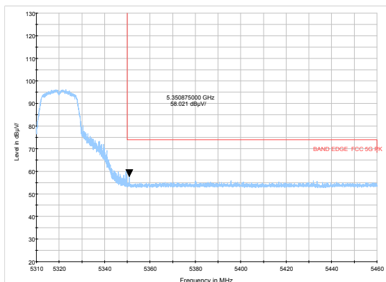
802.11a-Channel 64: Average
