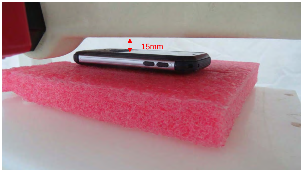
Picture 13: Front Side, the distance from handset to the bottom of the Phantom is 15mm
