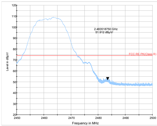
802.11b-Channel 11 Peak
