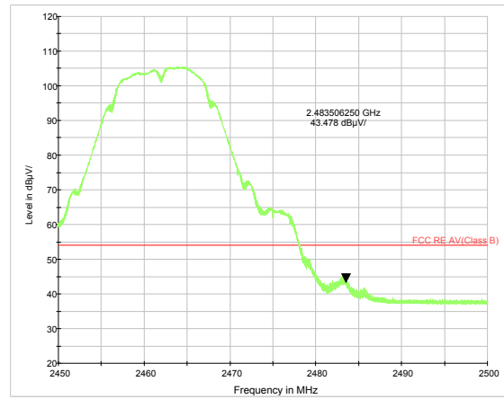
802.11b-Channel 11 Average
