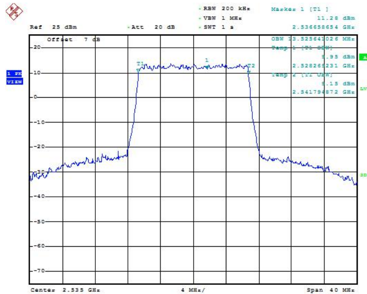
Fig.29 LTE band 7, 15MHz Bandwidth, QPSK (99% BW)
