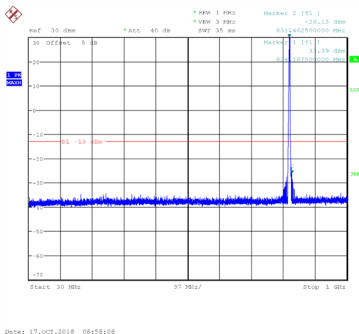
Fig.65 Channel 128: 30MHz~1GHz
