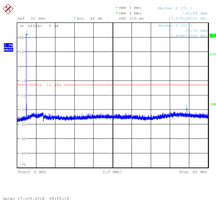
Fig.82 Channel 9538: 1GHz~20GHz
