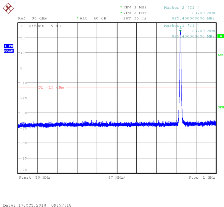
Fig.83 Channel 4132: 30MHz~1GHz
