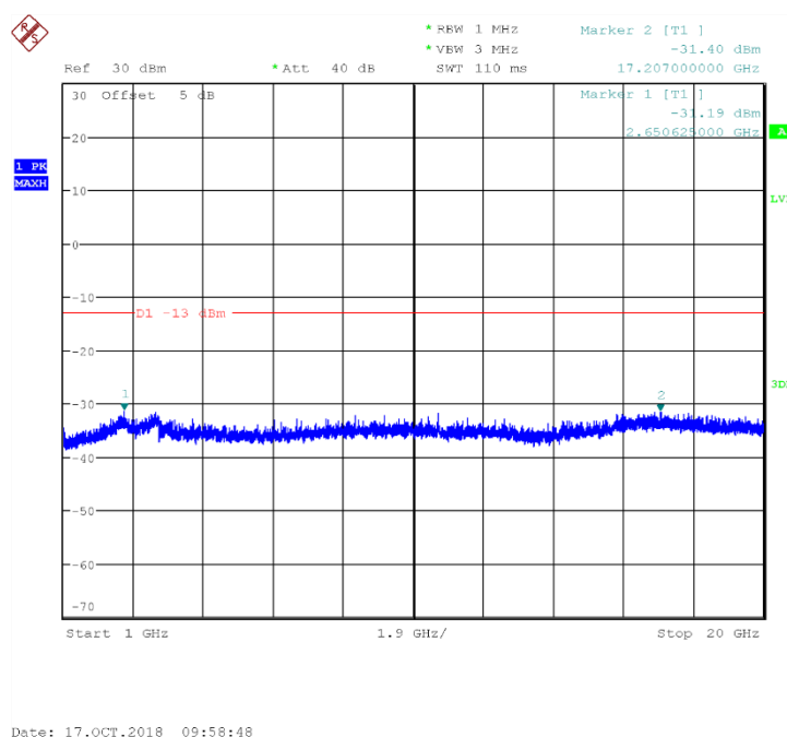
Fig.88 Channel 4233: 1GHz~20GHz
