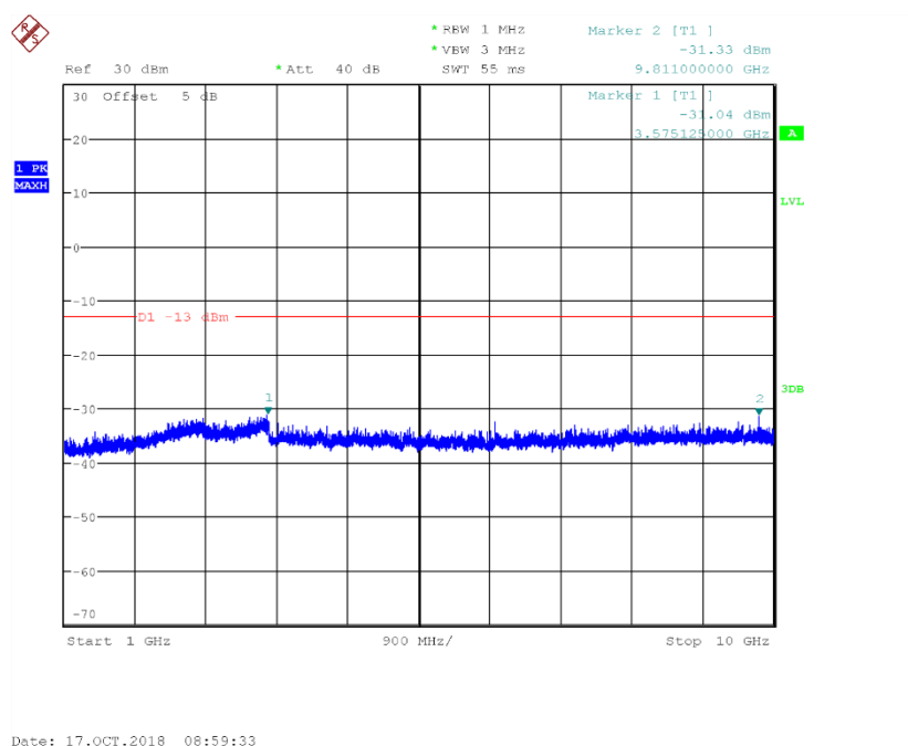
Fig.70 Channel 251: 1GHz~10GHz
