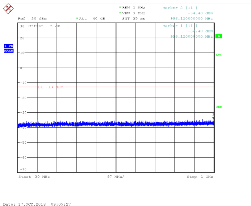
Fig.71 Channel 512: 30MHz~1GHz
