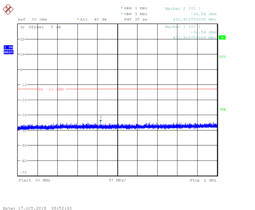
Fig.79 Channel 9400: 30MHz~1GHz
