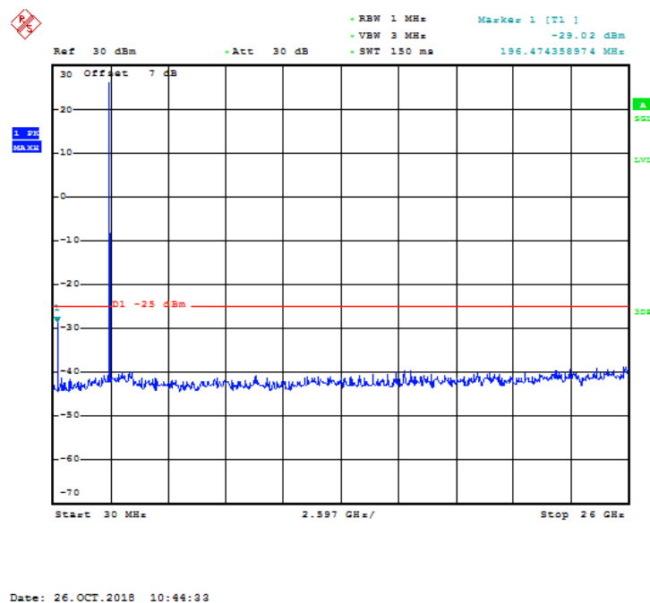
Fig.45 LTE band 7: 30MHz – 26GHz
