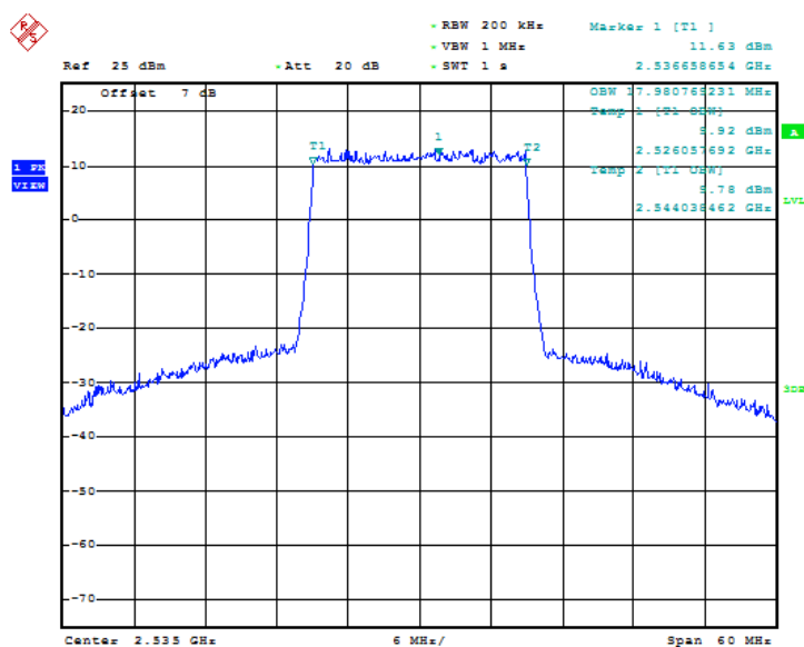
Fig.31 LTE band 7, 20MHz Bandwidth, QPSK (99% BW)
