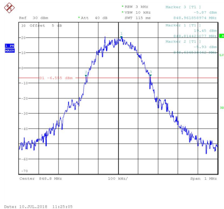
Channel 251- Emission Bandwidth (-26dBc BW)
