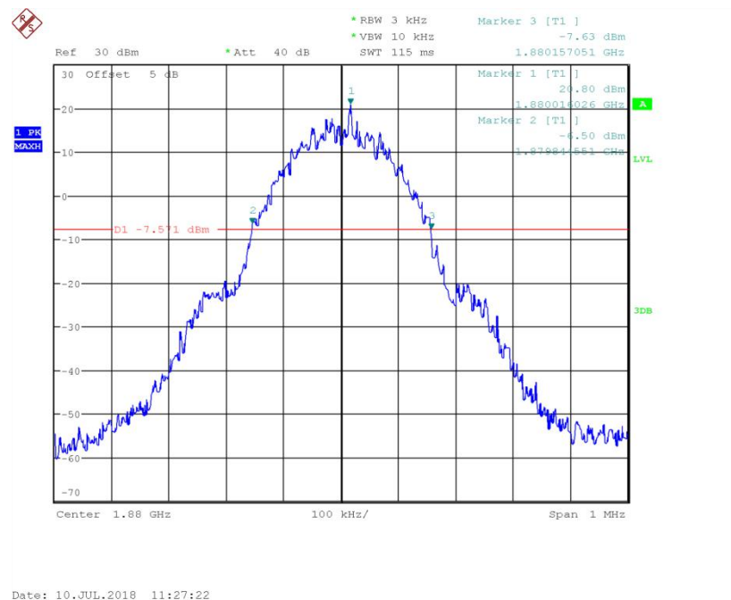
Channel 661- Emission Bandwidth (-26dBc BW)
