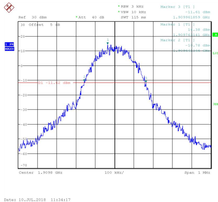
Channel 810- Emission Bandwidth (-26dBc BW)
