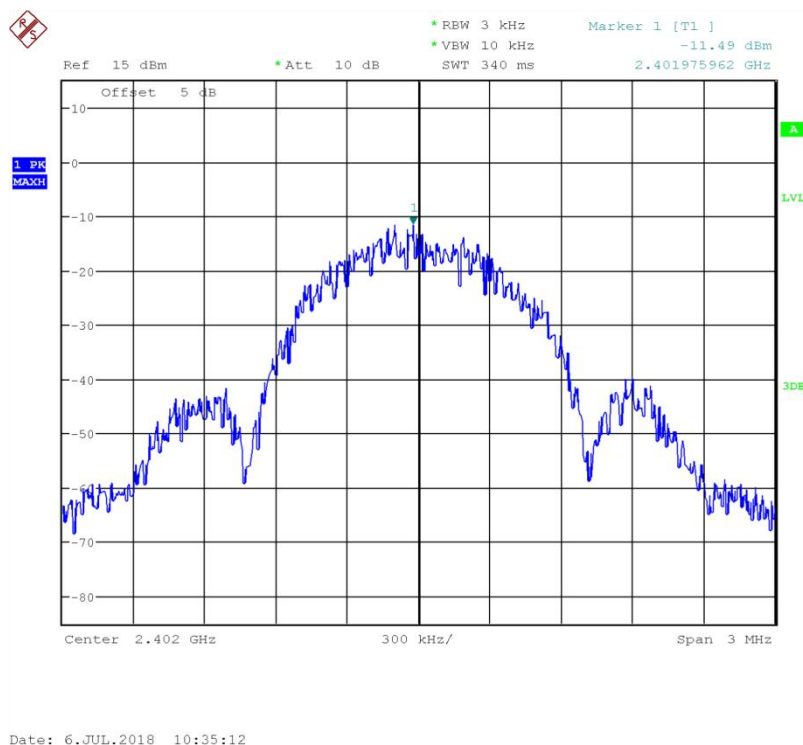
Fig.4 Power spectral density: CH0
