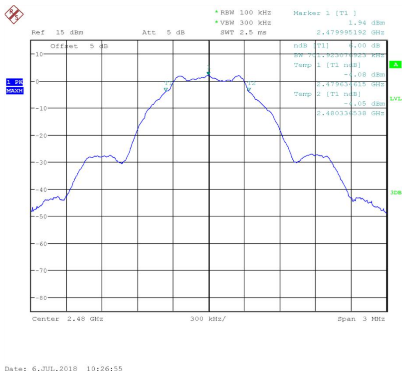
Fig.9 6dB Bandwidth: Ch39
