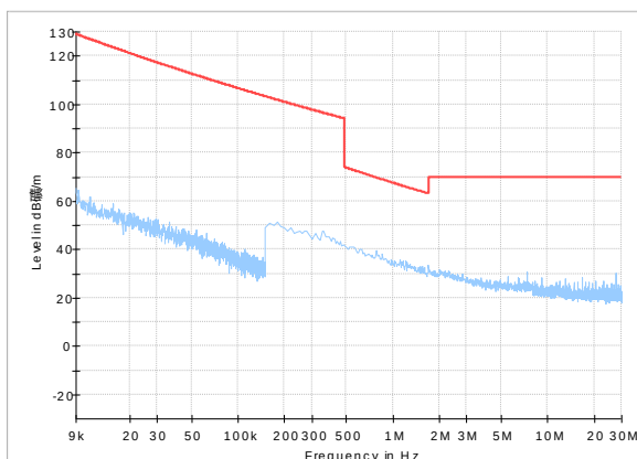
Radiated Spurious Emission (9kHz-30MHz)
