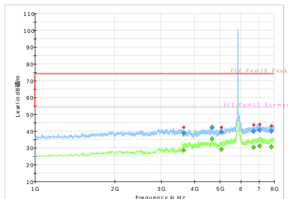
Radiated Spurious Emission (802.11a, ch165, 1GHz-8GHz)
