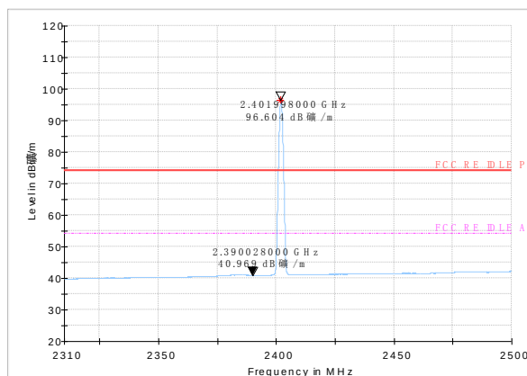
Bandedge: Ch0
