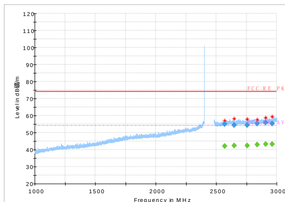
Bandedge: Ch0
