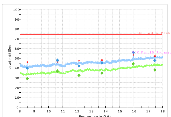
Radiated Spurious Emission (802.11a, ch64, 8GHz-18GHz)
