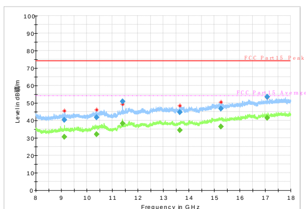
Radiated Spurious Emission (802.11a, ch140, 8GHz-18GHz)
