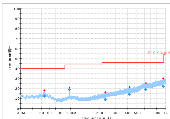
Radiated Spurious Emission (802.11a, ch140, 30 MHz-1 GHz)
