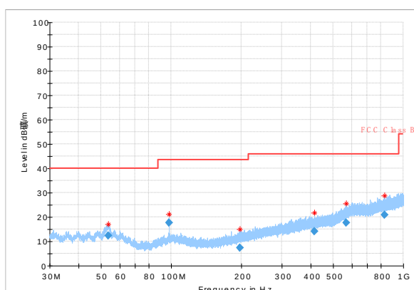
Radiated Spurious Emission (802.11a, ch64, 30 MHz-1 GHz)
