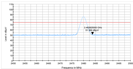
DH5-Channel 78: Peak
