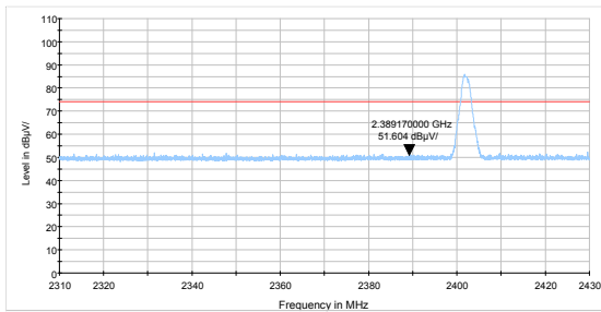
DH5-Channel 0: Peak
