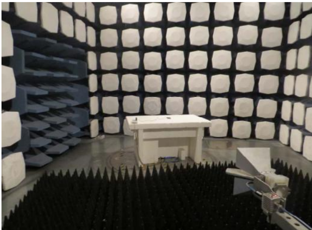
Picture 2 Radiated Spurious Emission Test Setup
