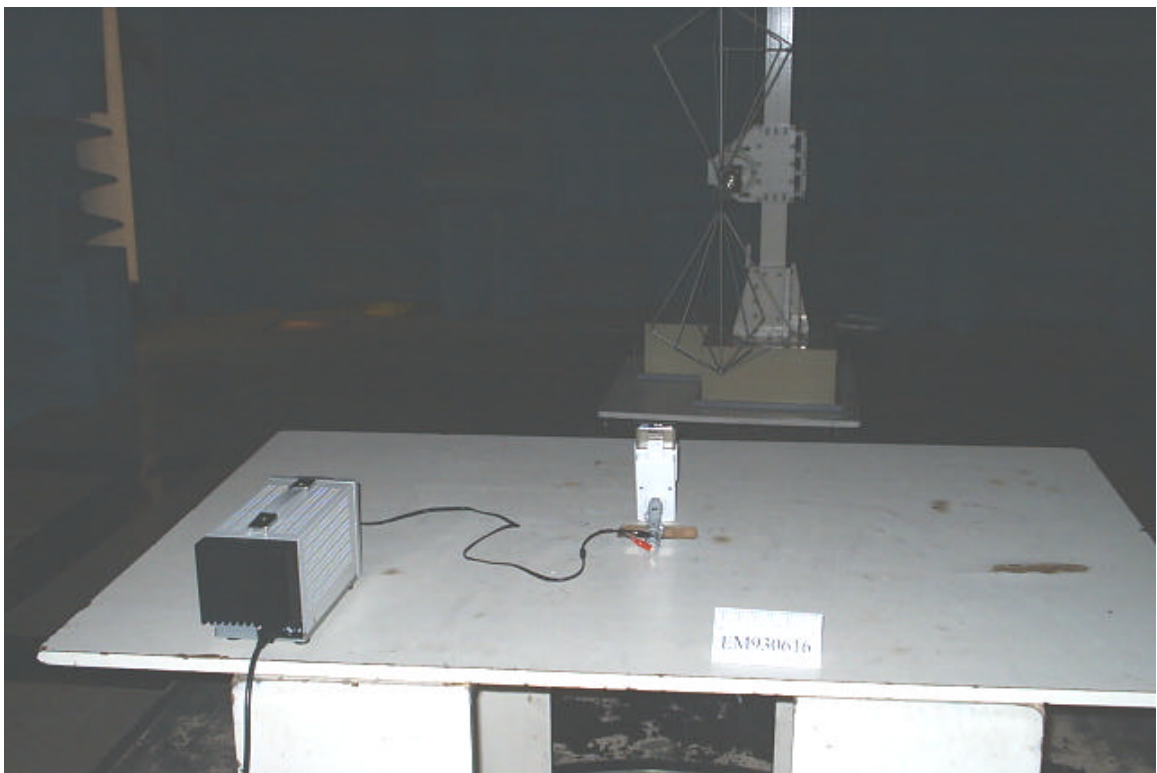
BACK VIEW OF RADIATED MEASUREMENT
