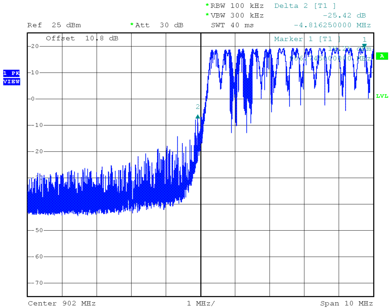
Plot 4.11 Conducted Band Edge (Hopping)
