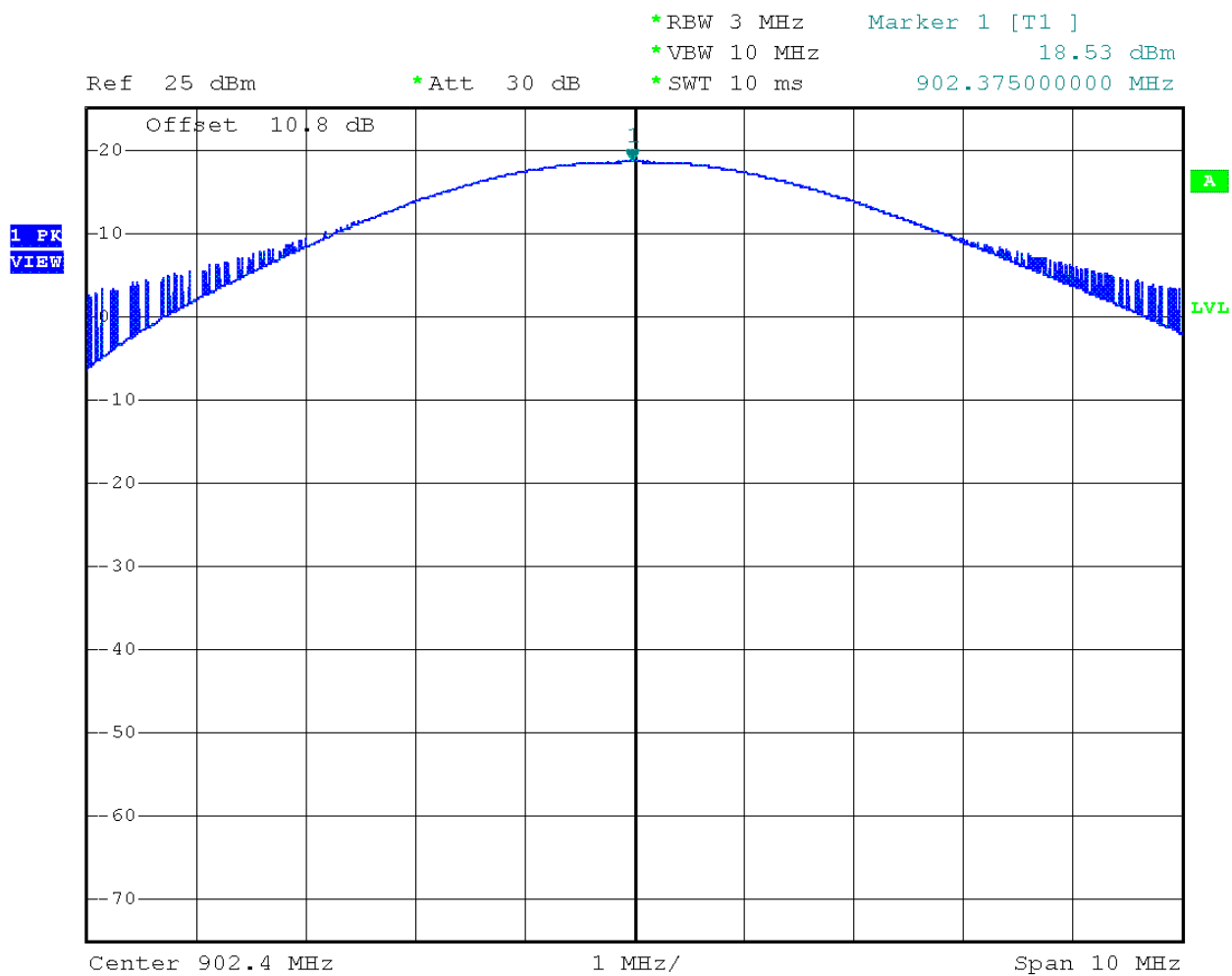
Plot 2. 2 – Output Power Low Channel
