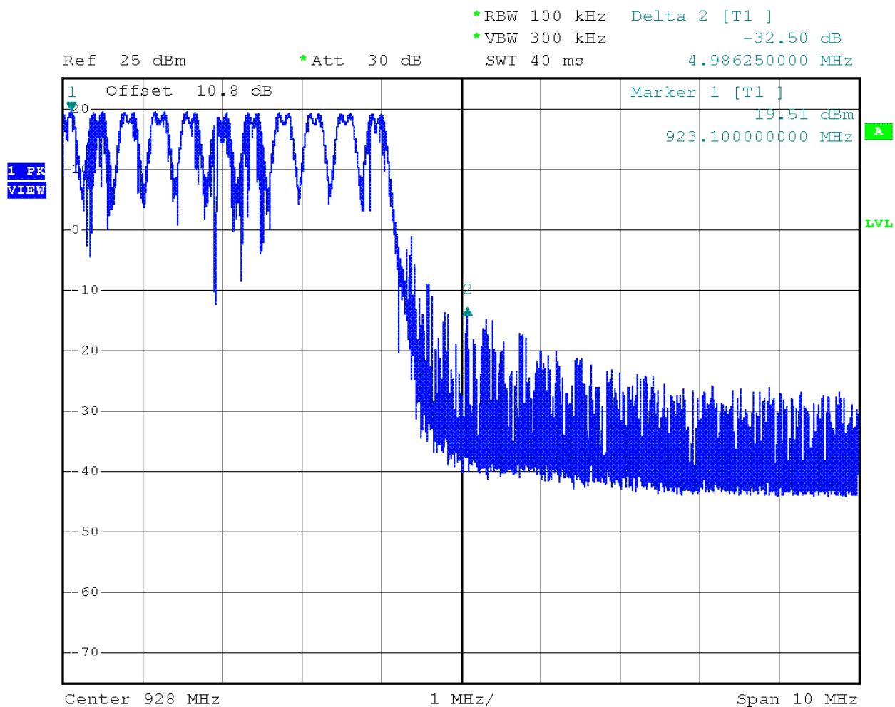
Plot 4.13 Conducted Band Edge (Hopping)
