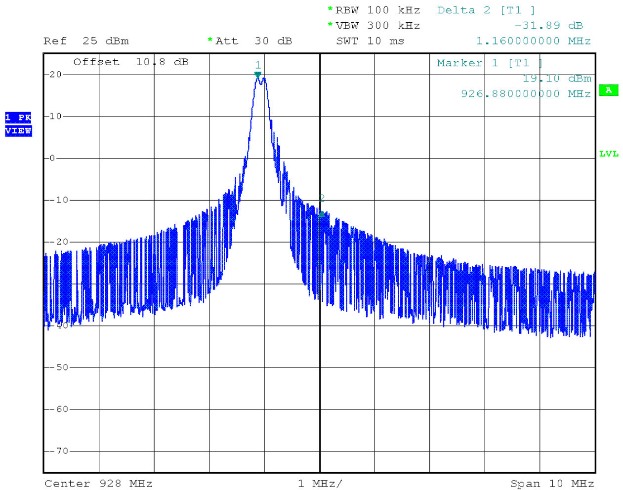
Plot 4.12 Conducted Band Edge, High Channel
