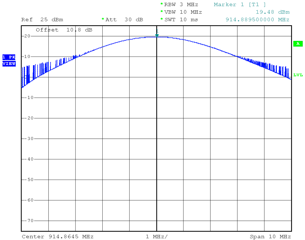
Plot 2. 2 – Output Power Middle Channel
