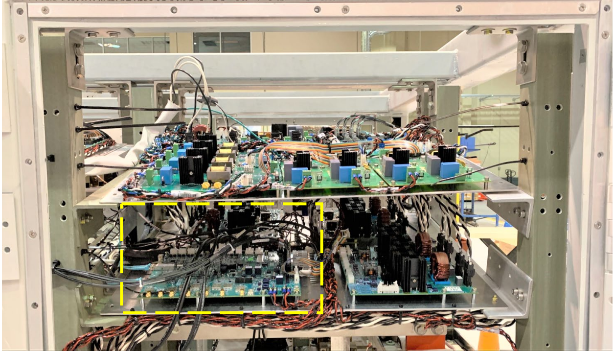
RF and control PCBA P110860 iDCE Board view 1
