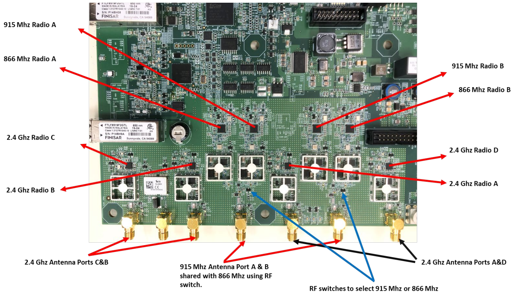
P110860 iDCE RF PCBA Radios (close up) EMC shields removed.
