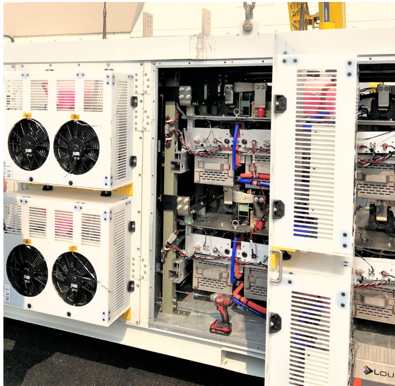
LCS side internal view
