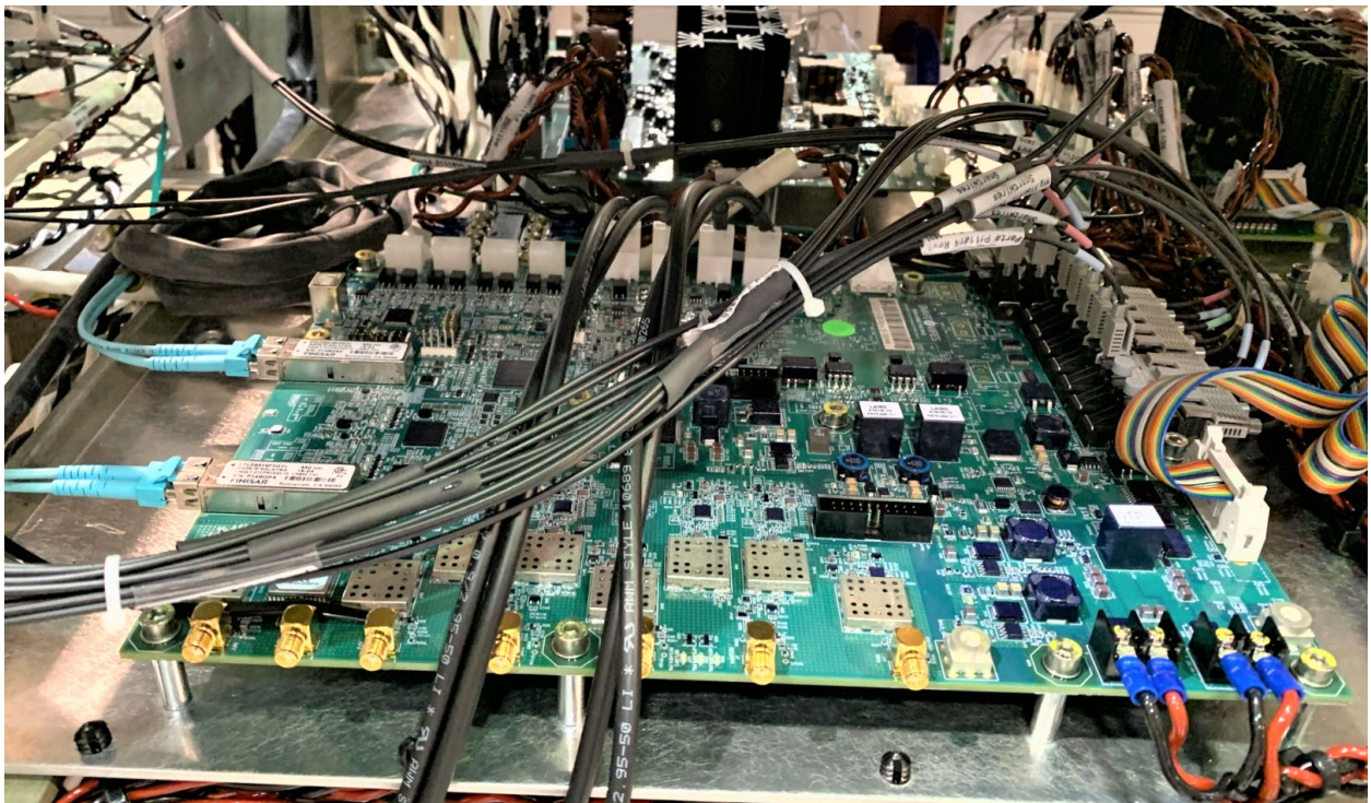
RF and control PCBA P110860 iDCE Board view 2
