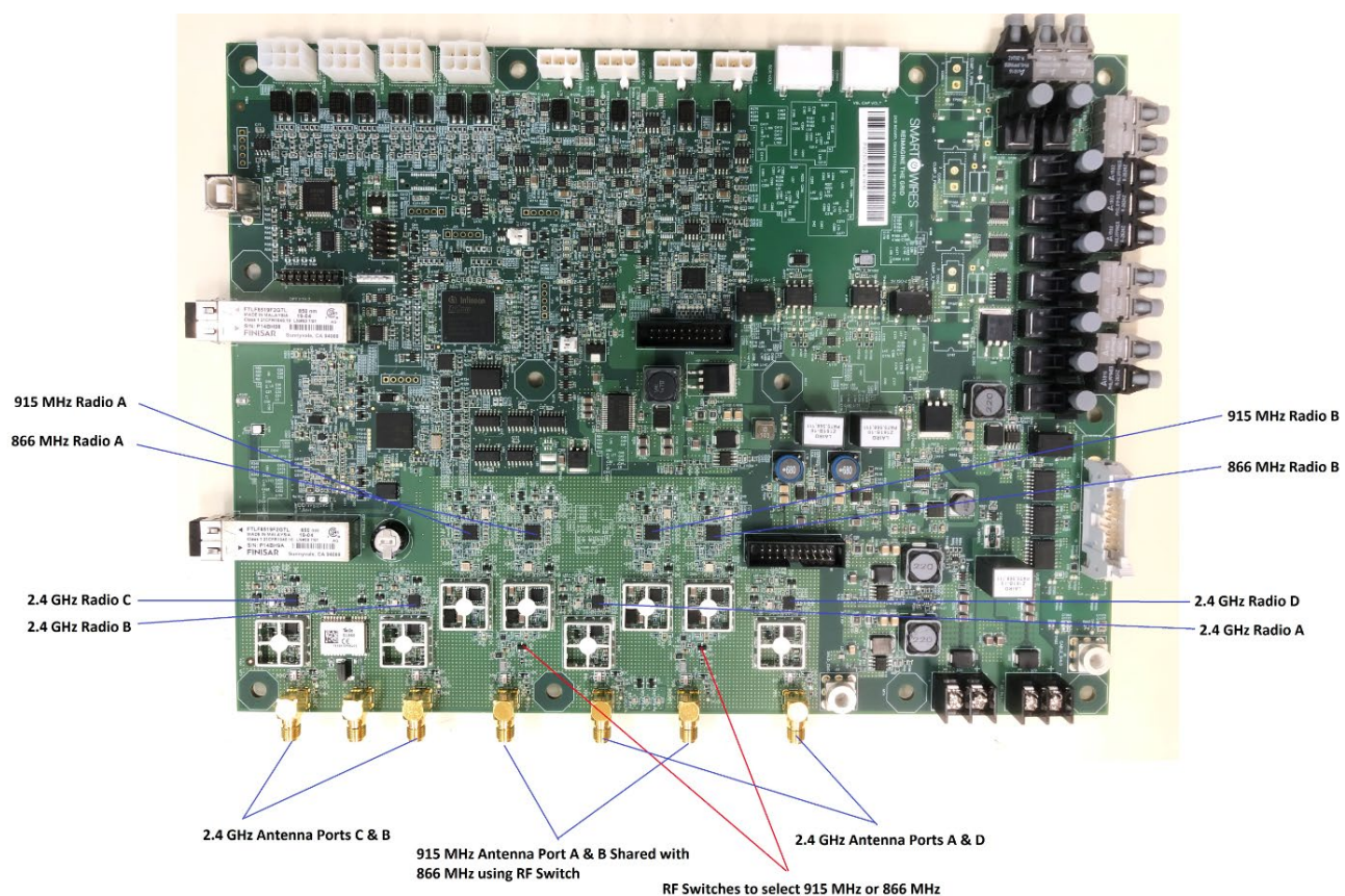
P110860 iDCE PCBA RF Layout (EMC shields removed)
