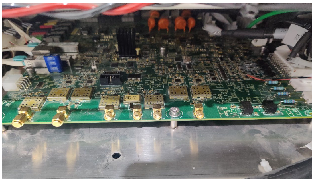
RF and control PCBA P110860 iiDCE Board view 2
