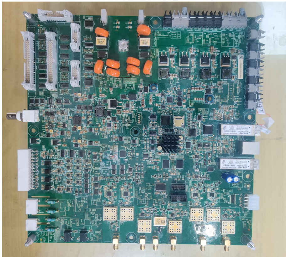
iiDCE PCBA RF Layout (EMC shields removed)
