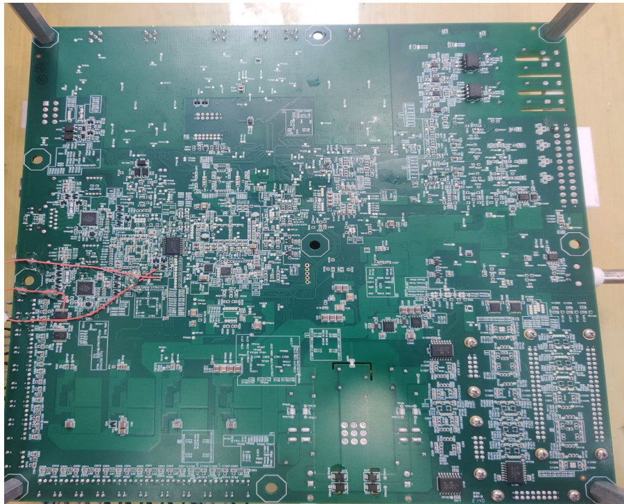
iiDCE (bottom view)
