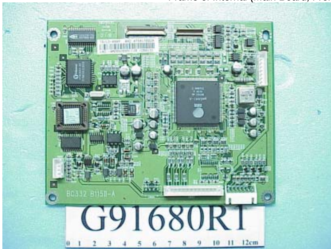
Figure 13 Frame of Internal (Main Board, Front Side)
