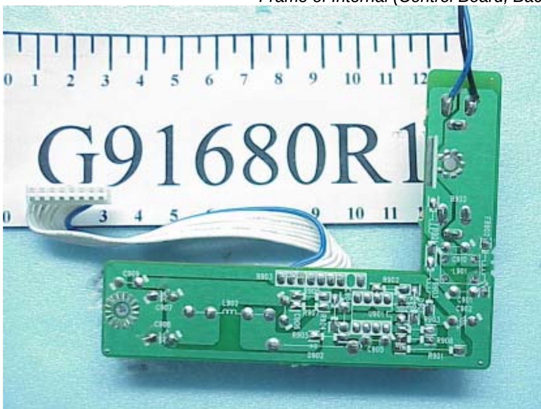
Figure 18 Frame of Internal (Control Board, Back Side)
