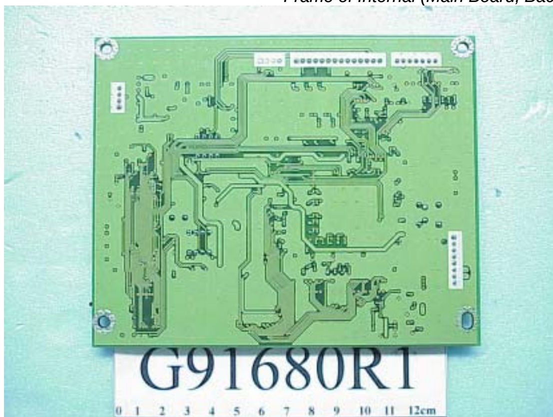
Figure 14 Frame of Internal (Main Board, Back Side)
