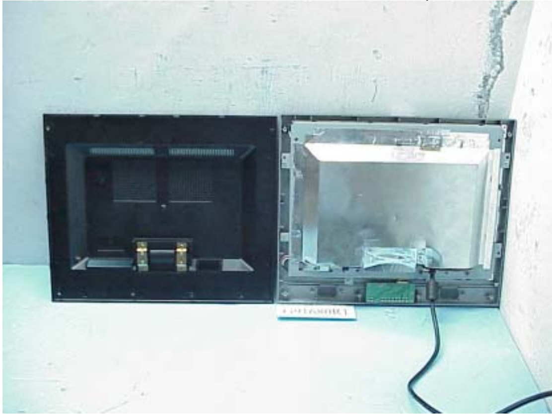
Figure 7 Internal View (Removed Back Cover)
