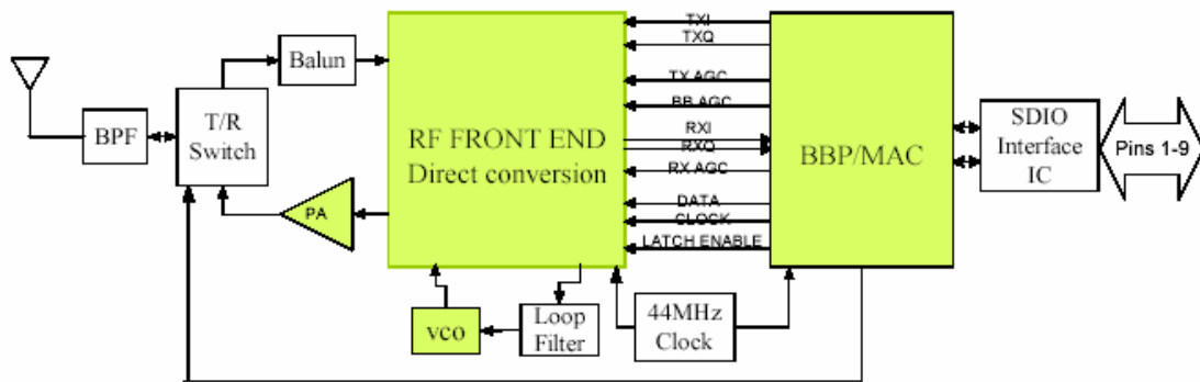
WLAN 6090SD NIC Block Diagram
