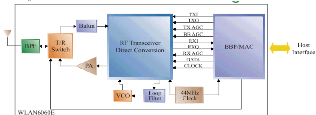
Figure 1. WLAN6060BB(EB) Block Diagram
