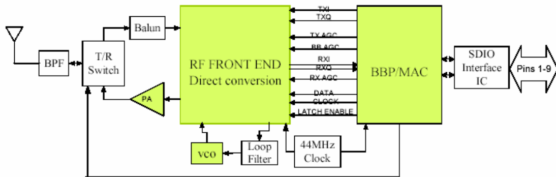
WLAN6060SD NIC Block Diagram
