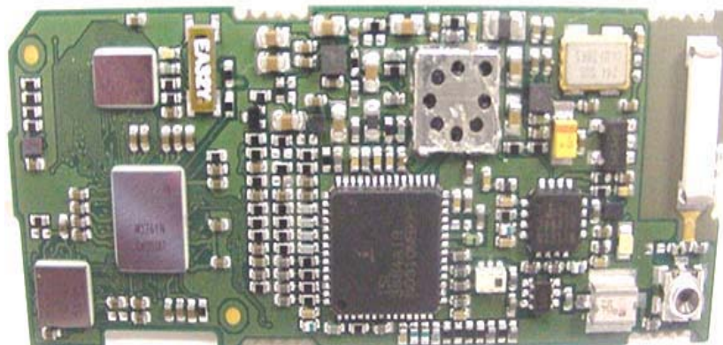
Front Side of EUT
