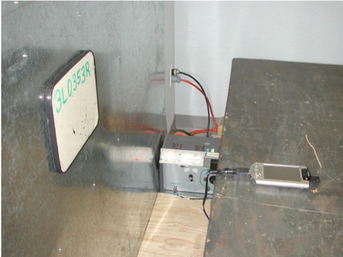
Powerline Conducted Emissions - Side
